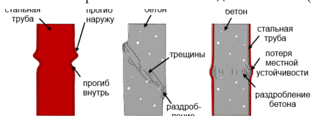
Fig. 2. Schematic failure modes of hollow steel tube, concrete and CFST stub columns
